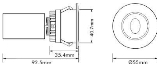
Cut-out: Ø45mm
