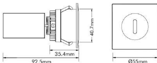
Cut-out: Ø45mm
