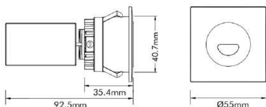
Cut-out: Ø45mm
