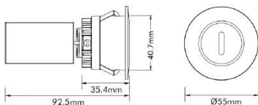
Cut-out: Ø45mm
