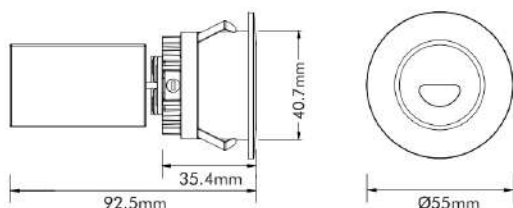
Cut-out: Ø45mm
