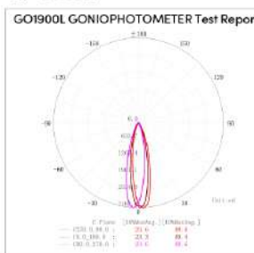
24°-3000K
