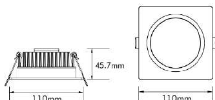
Cut-out: Ø90mm-100mm
