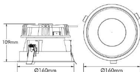
Cut-out: Ø150mm
