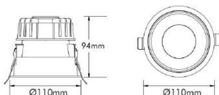
Cut-out: Ø100mm
